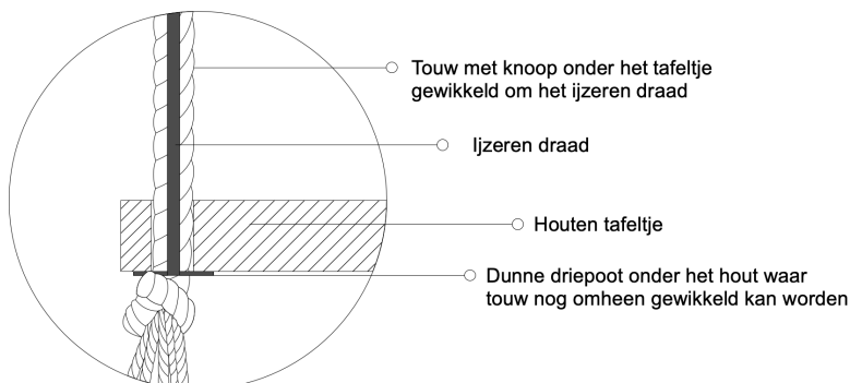
Detail C 2
